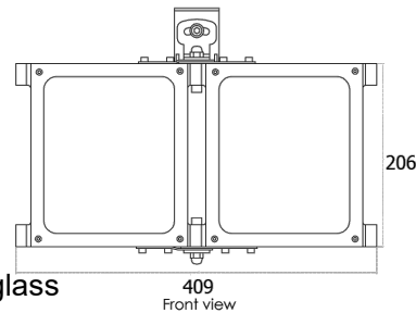
409 Front view
